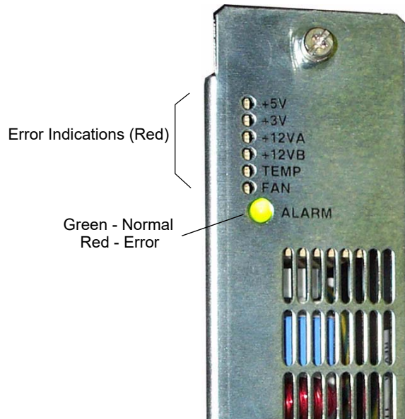
FIGURE 4-25. Power Supply
