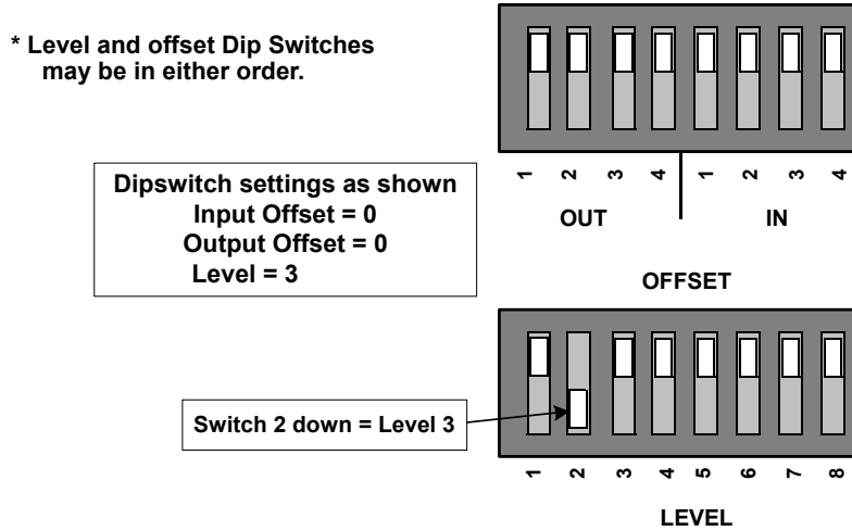
FIGURE 2-9. Utah-400 Configuration Dipswitches as they appear on the Crosspoint Carrier Board
