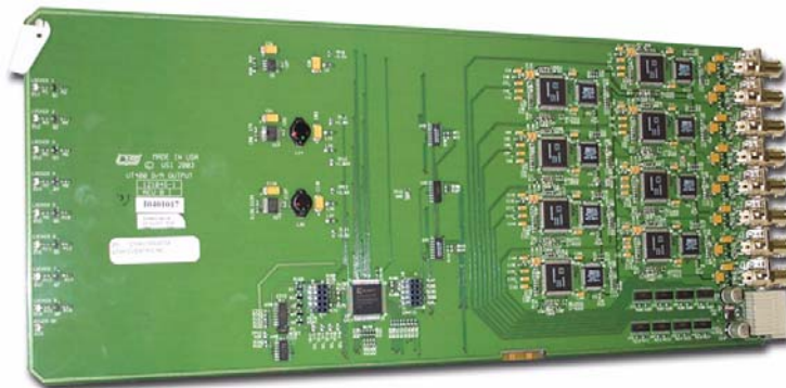
FIGURE 4-10. Digital to Analog Output Card
