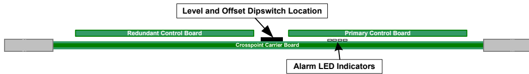
Crosspoint Board - Looking at the Front
