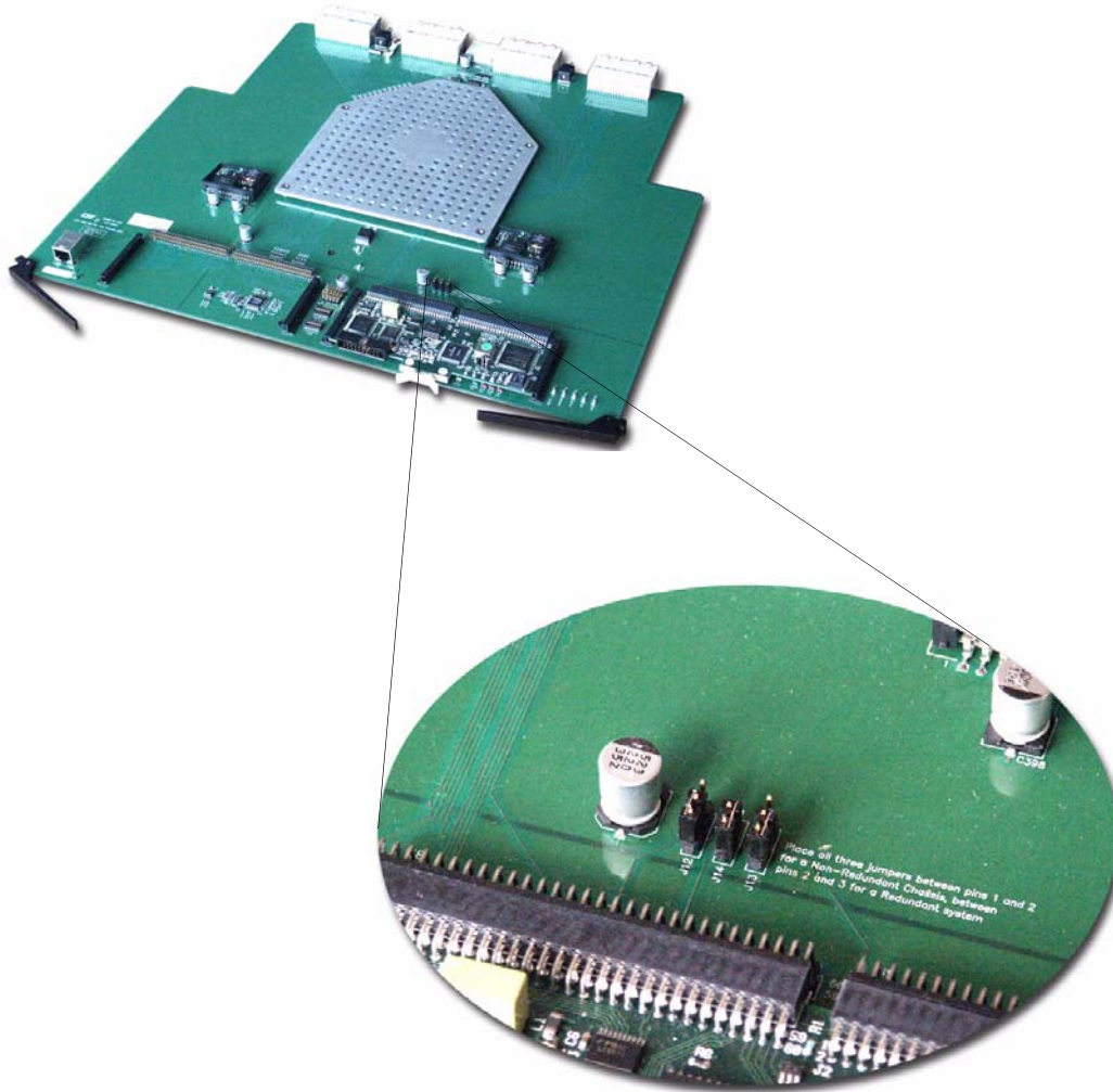
FIGURE 4-21. Video crosspoint module jumper location
