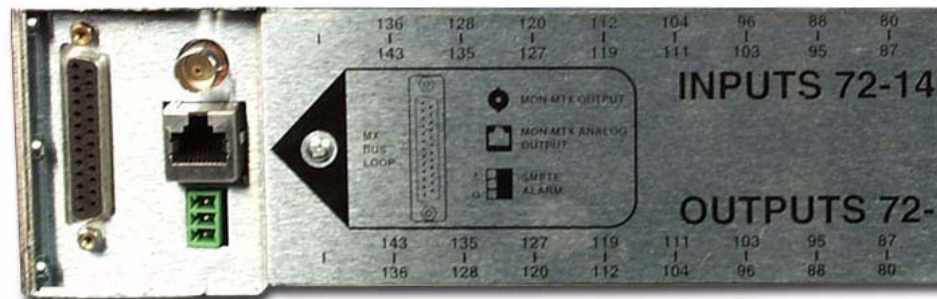
FIGURE 4-24. Audio Midplane's RJ-45 connection
